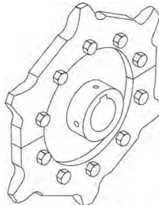
Removable Rim
