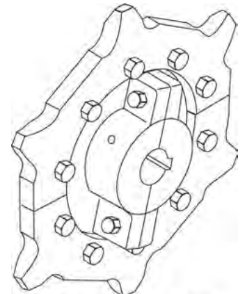
Split Removable Rim
